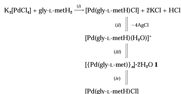
Scheme 1 (i) KOH, pH 2; (ii) 4AgNO 3 ; (iii) KOH, pH 6; (iv) HCl, pH 3
