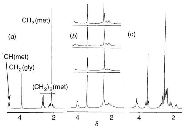
Fig. 2 Proton NMR spectra (δ 1.5–4.5) of gly-met at pD 2.4 in D 2 O, at 293 K (a), [Pd(gly-L-metH)Cl] in KCl, at pD 3 in D 2 O at 293, 289, 285 and 280 K (bottom to top) (b) and [Pt(gly-L-metH)Cl], at pD 4.8 in D 2 O at 293 K (c)
