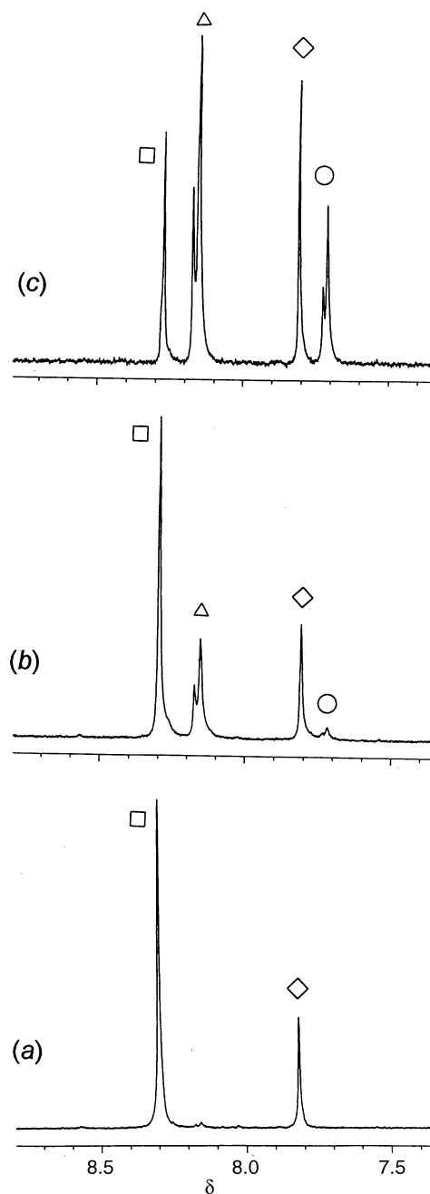
Fig. 3 9-Ethylguanine H 8 ( \delta 7.5–8.5) resonances of 1 : 1 mixtures of Hegua and complex 1 , c = 0.033 mol dm -3 , in D 2 O, at pD 5.6 (a), 7.0 (b) and 8.3 (c). The H 8 resonances are marked as follows: (◇) Hegua/egua; (□) Pd(Hegua-N 7 )/Pd(egua-N 7 ); (○) Pd(egua-N 4 ); (△) Pd 2 (egua-N 4 ,N 7 )
